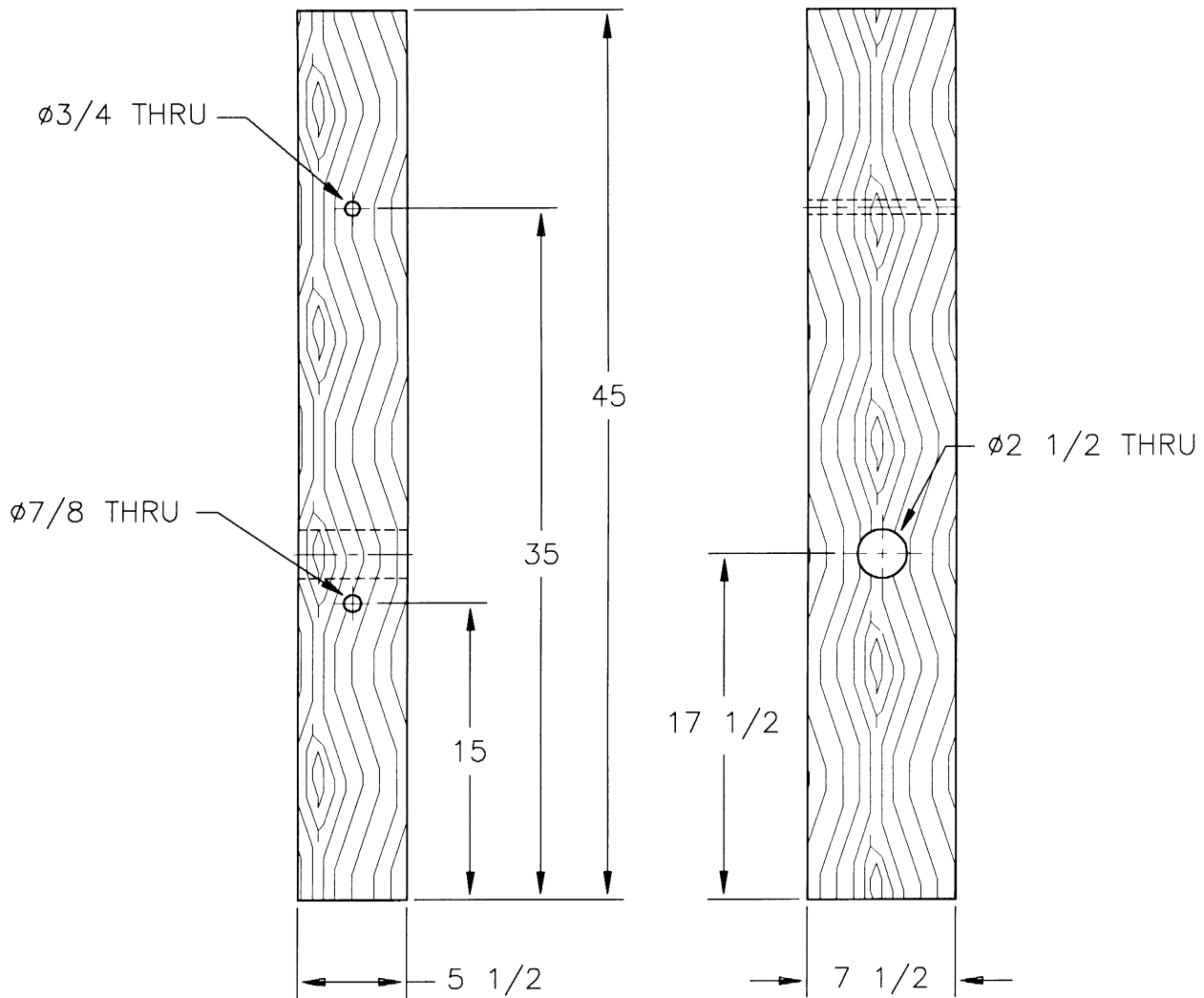
5 \frac{1}{2} \times 7 \frac{1}{2} \times 45 WOOD BREAKAWAY POST
