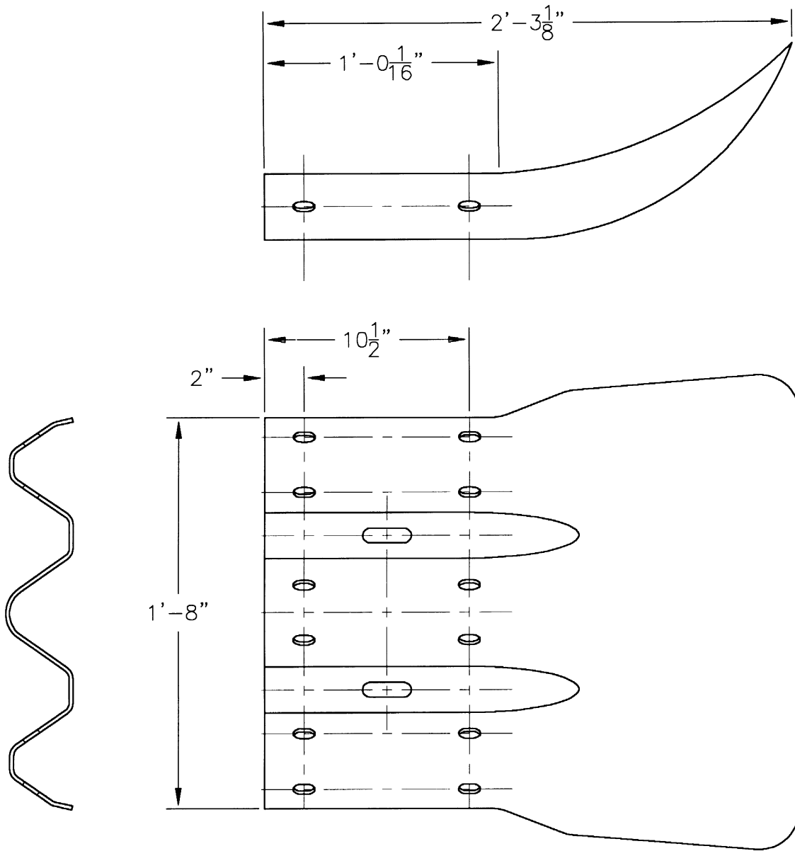
12GA/THRIE BEAM FLARED END
