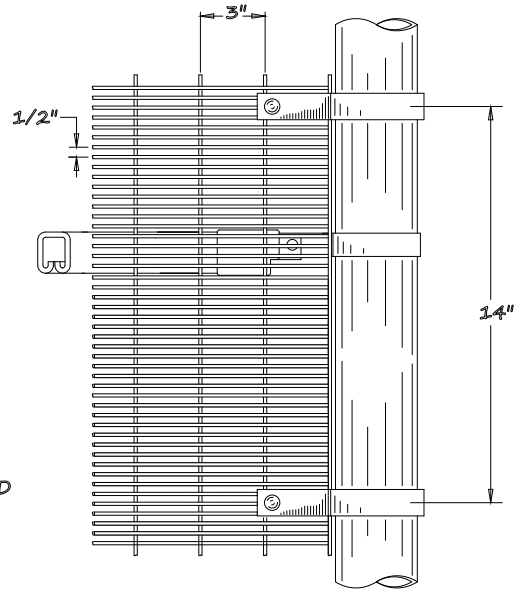
END/CORNER CONNECTION
